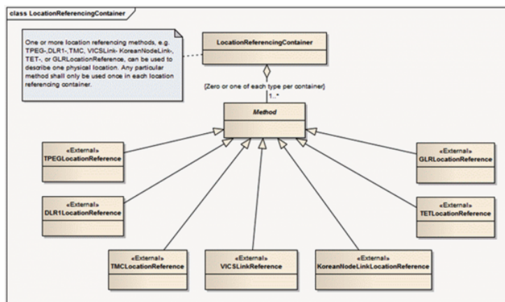
Obrázek 2 - Location Referencing Container construct
