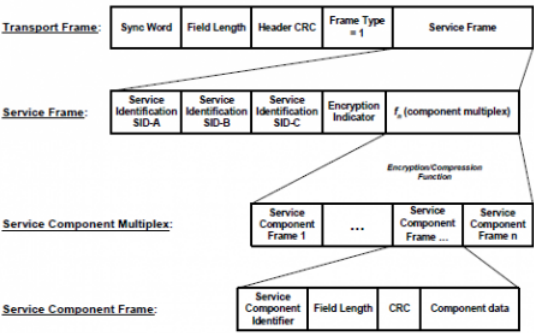
Figure A.3 — TPEG Frame Structure, Frame Type = 1 (i.e. conventional data)
