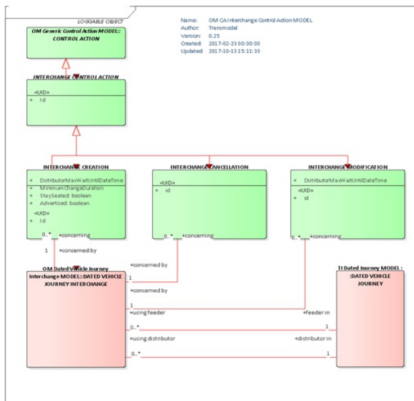
Figure C.11 — TRM6_CR_OM— 010 Proposed Interchange Control Action MODEL
